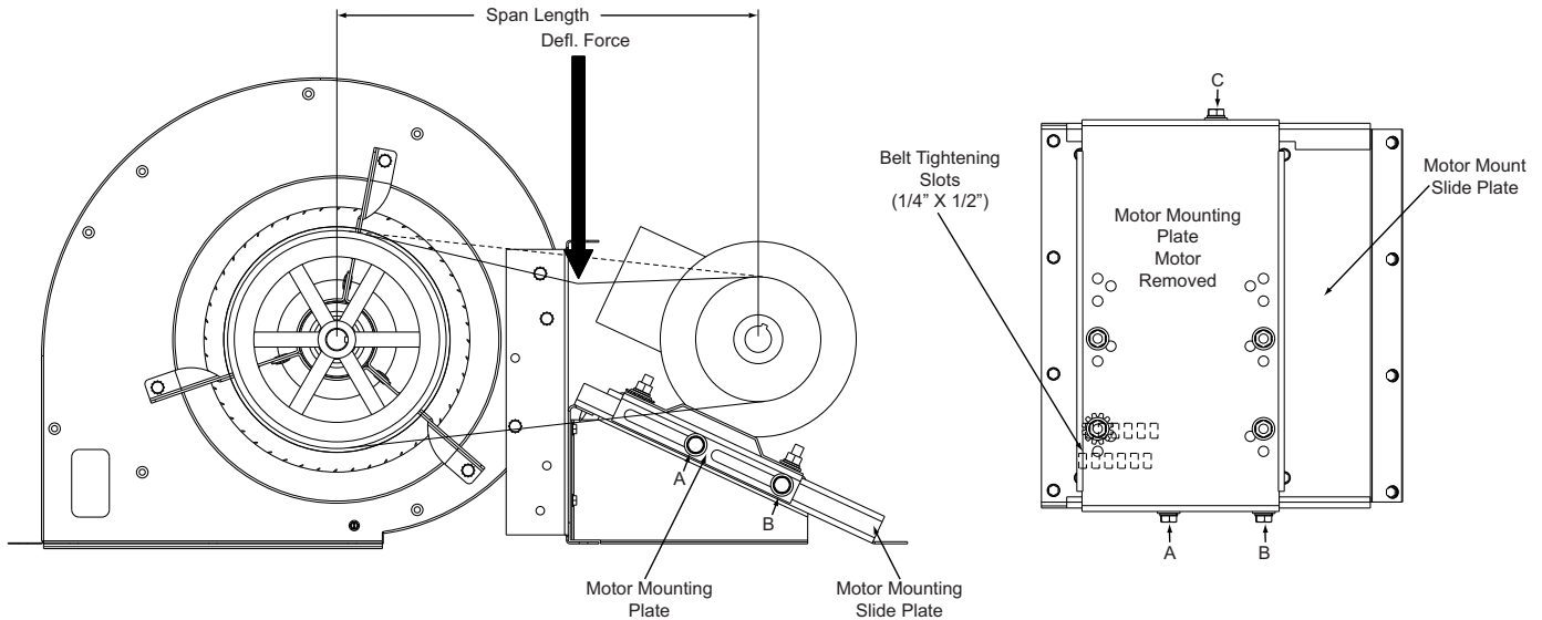
Figure 22: Belt Adjustment
