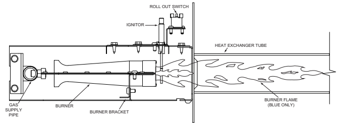
Figure 27: Typical Flame
